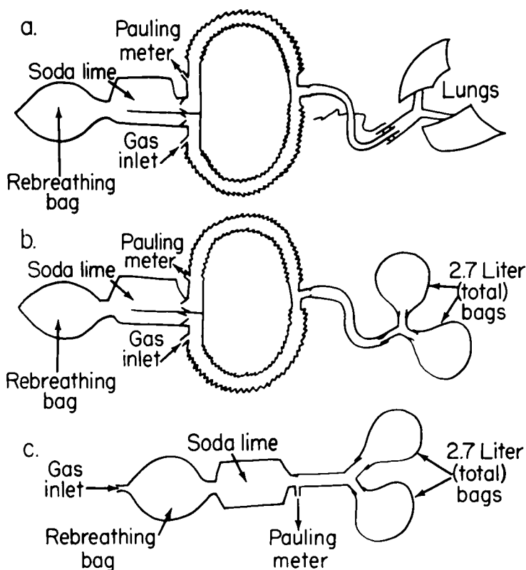
FIG. 1. A. Diagrammatic representation of the combined circle system and patient showing the physical arrangement, the points of gas inflow and of gas exit for sampling. The gas exit for overflow (not shown) is at the usual point just before the expiratory valve. B. The same system with the substitution of a 2.7-liter "lung" composed of two rubber bags for the patient's lungs. C. A to-and-fro system is substituted for the circle system, the 2.7-liter "lung" being retained. The gas exit for overflow (not shown) lies at the same point as the exit for the Pauling meter.
