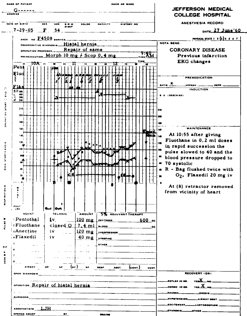
FIG. 2. Anesthesia record illustrating production of hypotension by overdose of halothane. Each short crosshatch represents 0.2 ml. of halothane.
