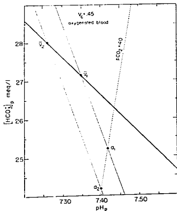
FIG. 2. Normal in-vitro \text{CO}_2 titration curve of true oxygenated mixed venous plasma ( \bar{v}_1 \bar{v}_2 ). a_1 and \bar{v}_1 represent plasma compositions of, respectively, arterial and mixed venous blood at control conditions; a_2 and \bar{v}_2 plasma compositions after reduction of cardiac output to half normal. The detailed blood compositions are given in table 2. For discussion see text.
