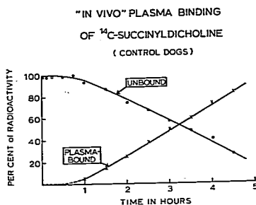
FIG. 7. Equilibrium dialysis of samples of plasma from control dogs, subsequent to the intravenous administration of ^{14}\text{C} -succinylcholine. Each value is the average of five experiments. Plasma proteins gradually bind ^{14}\text{C} -succinylcholine and its metabolites. The binding, however, is negligible during the first 45 minutes after injection, even though a high concentration of labeled materials is present in plasma during this interval. Five hours after injection, 84 per cent of the total plasma radioactivity is bound to plasma.
