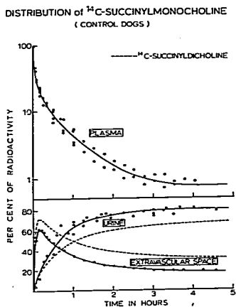
FIG. 3. Disappearance from plasma, cumulative urinary elimination, and passage into the extravascular space of radiocarbon ( ^{14}\text{C} ), subsequent to the intravenous administration of ^{14}\text{C} -succinylmonochohline to control dogs.
