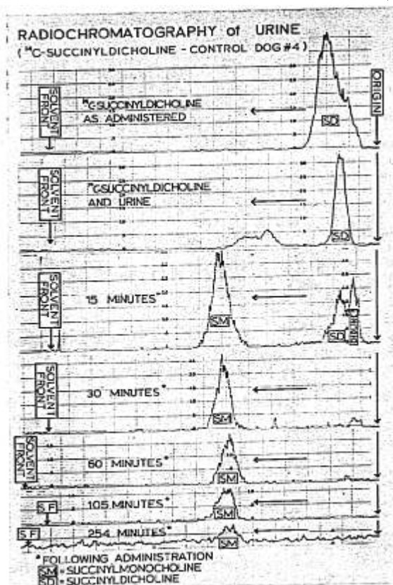
FIG. 5. Paper radiochromatograms of 14 C-succinylcholine as administered, 14 C-succinylcholine added to a sample of normal urine, and samples of urine subsequent to intravenous administration of 14 C-succinylcholine.
