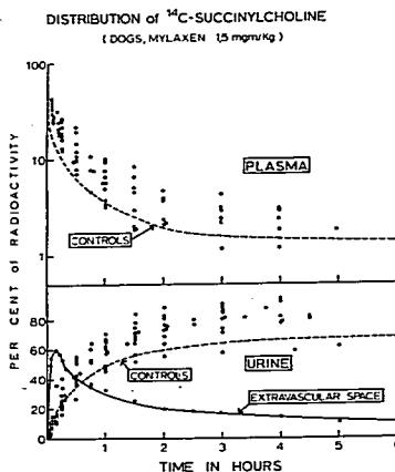
FIG. 4. Disappearance rate from plasma, urinary elimination, and passage into the extravascular space of ^{14}\text{C} of a trace dose of ^{14}\text{C} -succinylcholine intravenously administered to dogs pretreated with hexafluorenum 1.5 mg/kg.
