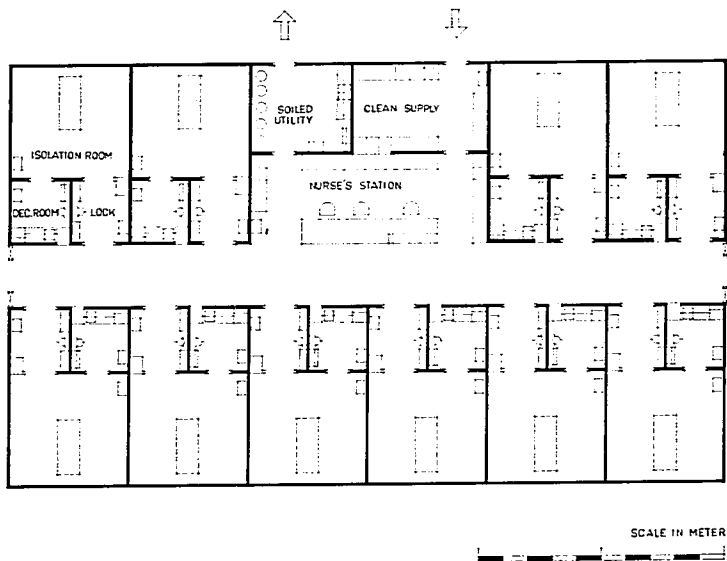
FIG. 5. A 10-bed intensive therapy unit with all beds in isolation rooms. The unit is one of four, planned for the new Huddinge Hospital, Sweden, a 1,600-bed hospital. (Architects, H.L.S. Medical advisers, Å. Wählin, O. von Dardel, P. E. Wiklund.) (Permission for reproduction obtained from authors. 4 )
