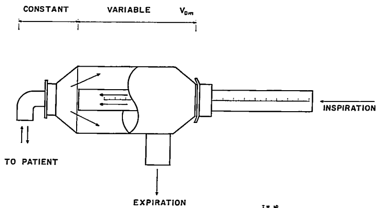
FIG. 1. Variable-deadspace device.
