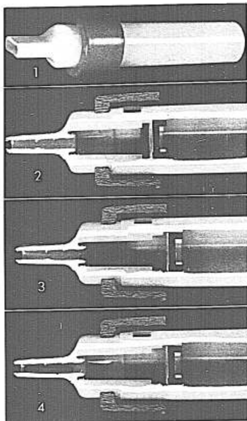
FIG. 1. The disposable nonrebreathing mouthpiece for the Juno Mark 2.
