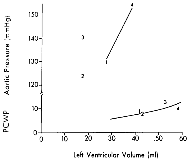
FIG. 1. Effect of reduced resistive load on left ventricular volume (abscissa, ml)-aortic-PCWP pressure (ordinate, mmHg) relationships. The numbers denote the four sequential experimental conditions, and indicate the mean pressure-volume coordinates for the six dogs in which measurements were obtained in all conditions. Stroke volume is the difference between diastolic and systolic values for each condition. The end-diastolic values in the lower right do not obviously depart from a single curve. The end-systolic coordinates with closed shunts (1-4) demonstrated that ESV increases from 1 to 4 (continuous lines) in our experiments. Note that the corresponding coordinate with open shunts (2 and 3) are displaced to the left of the continuous lines, indicating reduced end-systolic volume at a given end-systolic pressure.
