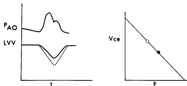
FIG. 5. Effect of reduced systemic vascular resistance on v_{ce} . Left Panel: Left ventricular volume decreases faster and farther when the shunt is open (interrupted line) than when it is closed (continuous line), and the corresponding aortic pressure traces are identical because higher flow occurs through lower resistance when the shunt is open. Right Panel: v_{ce} (ordinate) varies inversely with load (F, abscissae) for a given contractile state. Because F is proportional to the volume-pressure product, it is less throughout ejection when the shunt is open (○) because ventricular volume is less at the same pressure than when the shunt is closed (●). Accordingly, v_{ce} increases at the same contractile state when the shunt is open.
