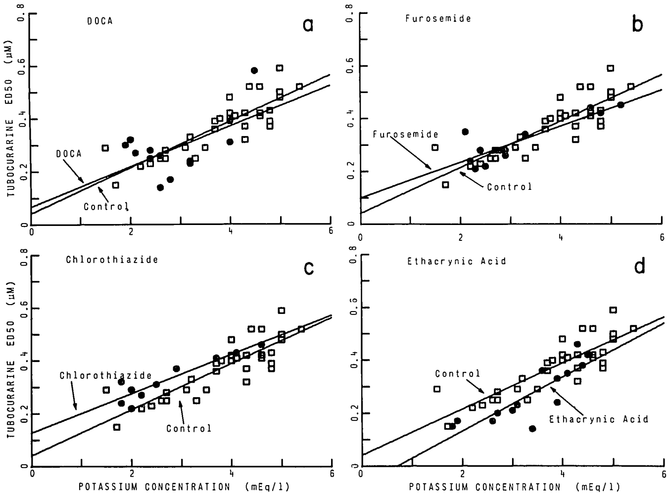
FIG. 2. Effects of DOCA (n = 13), furosemide (n = 12), chlorothiazide (n = 10), and ethacrynic acid (n = 14) on ED 50 of tubocurarine. Ordinates and abscissae as in figure 1. Circles: values obtained when drug indicated was added to the dietary pretreatment. DOCA and furosemide produced no effect beyond that seen with diet alone while chlorothiazide produced slightly less and ethacrynic acid slightly more reduction in tubocurarine ED 50 as the potassium concentration fell.
