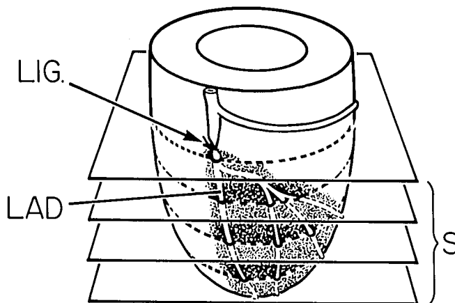
FIG. 1. The figure schematically represents the left ventricle and shows the left anterior descending (LAD) coronary artery, the site of LAD ligation (LIG), the extent of ischemic myocardium (shaded area), and the planes of sectioning (S).
