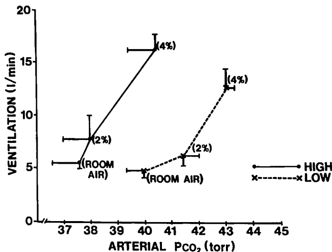
FIG. 1. The V E ·PaCO 2 relationship is shown (mean ± SEM). With increasing N intake, there was a leftward shift of the V E ·PaCO 2 regression. The concentration of administered CO 2 is noted in parentheses.
