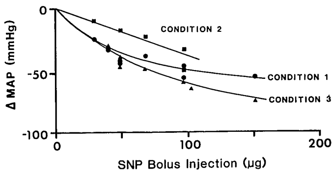
FIG. 3. MAP dose response curves to sodium nitroprusside before phenylephrine (Condition 1, ●), during 40 µg/min phenylephrine (Condition 2, ■), and after stopping phenylephrine (Condition 3, ▲) for the same experiment illustrated in Figure 2. The dose response curves were computed as in Figure 2.
