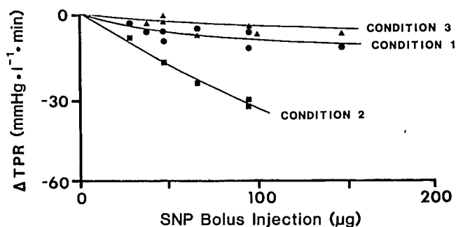
FIG. 2. TPR dose response curves to sodium nitroprusside before phenylephrine (Condition 1, ●), during 40 µg/min phenylephrine (Condition 2, ■), and after stopping phenylephrine (Condition 3, ▲) for one experiment. The dose-response curves were computed by least-squares fitting of a Michaelis-Menten equation to the experimental data.
