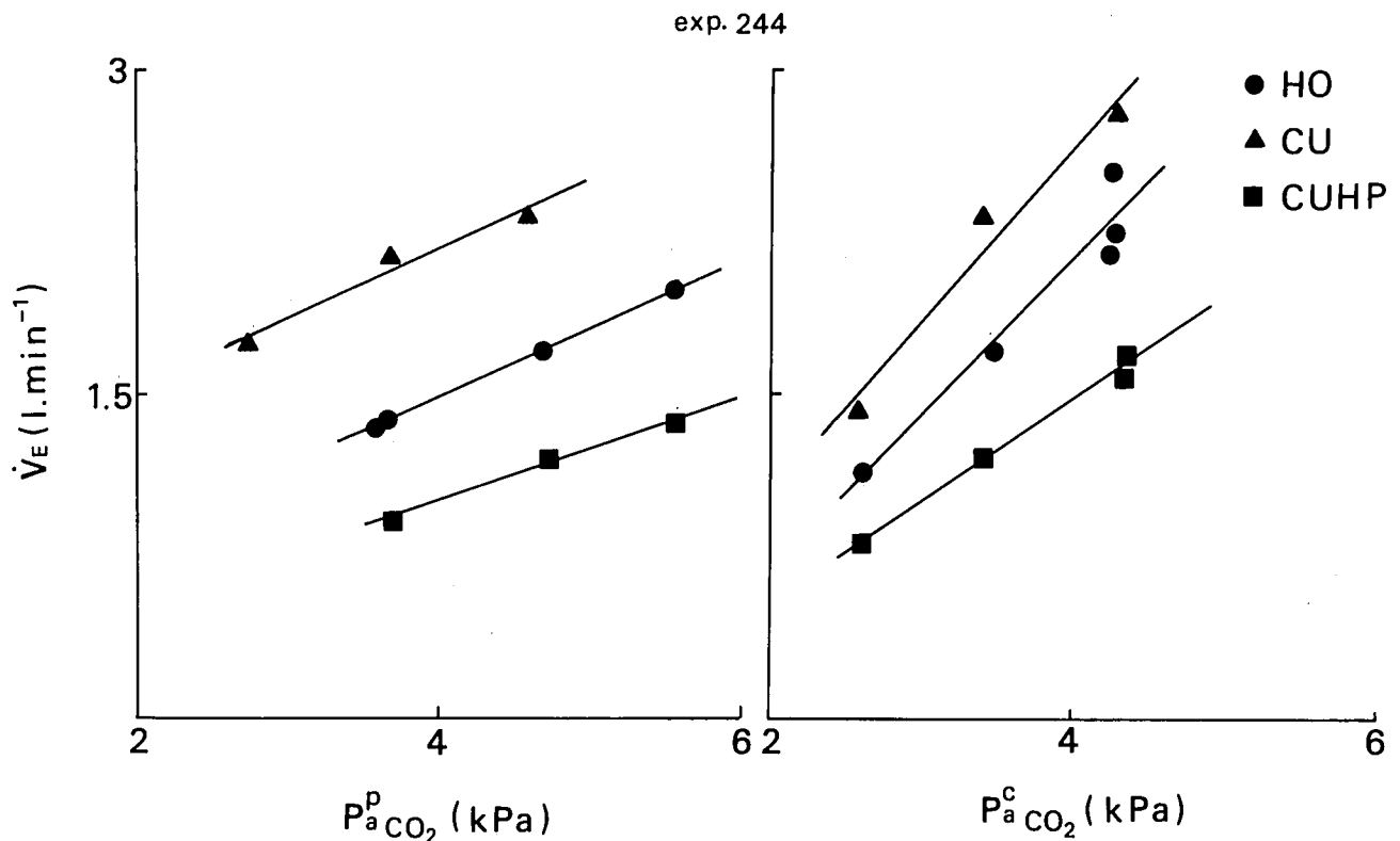
FIG. 4. Ventilatory responses during artificial brain stem perfusion to changes in peripheral P aCO 2 p (left panel) at constant central P aCO 2 (3.3 kPa; 25 mmHg) and to changes in central P aCO 2 c (right panel) at constant peripheral P aCO 2 (4.7 kPa; 35 mmHg). The peripheral P aO 2 was kept constant at 7 kPa (53 mmHg), the central P aO 2 at 50 kPa (375 mmHg) during halothane anesthesia overall (HO), chloralose–urethane (CU), and chloralose–urethane anesthesia with halothane added peripherally (CUHP).
