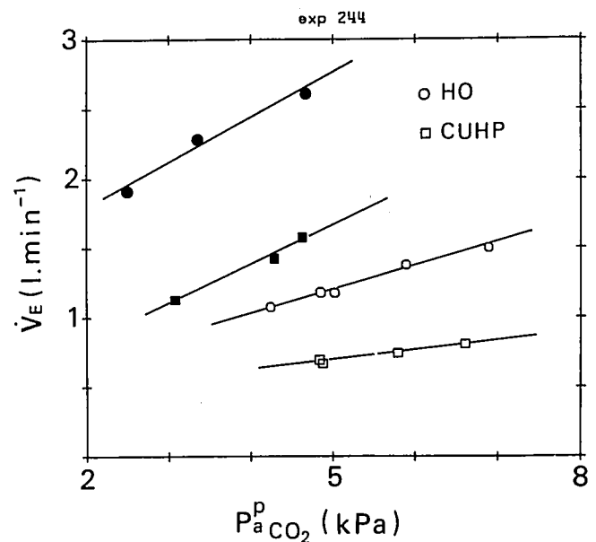
FIG. 5. Ventilatory responses to changes in peripheral PaCO 2 during peripheral hyperoxia ( open symbols ) and peripheral hypoxia ( closed symbols ) illustrated in one cat during halothane overall (HO) and chloralose-urethane anesthesia with halothane added peripherally (CUHP). The central PaCO 2 was kept constant at 4.1 kPa (31 mmHg) and the central PaO 2 at about 50 kPa (375 mmHg).
