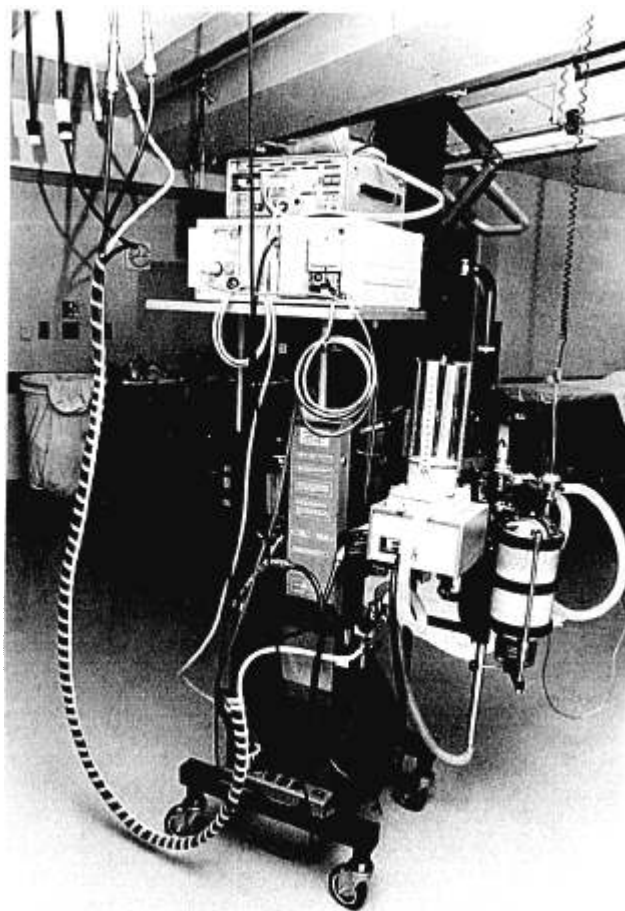
FIG. 1. Illustration of gas, vacuum, and electrical supply to an anesthesia machine.
