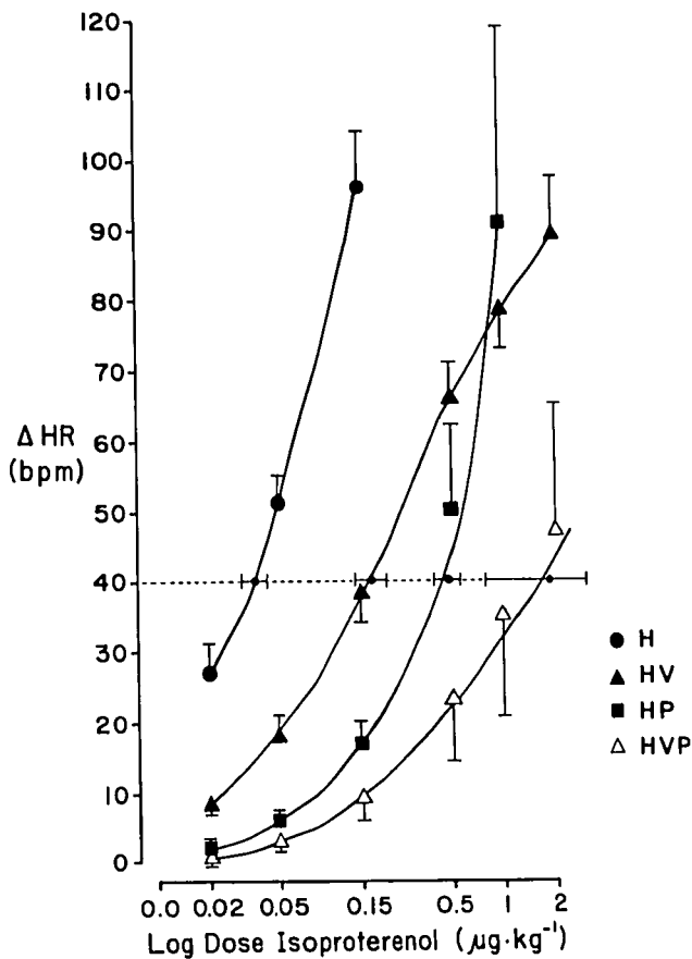
FIG. 3. Semilogarithmic plot of the isoproterenol dose versus the means of the maximal change in heart rate for groups H, HP, HV and HVP for period 2. Heart rate values interpolated from the individual double reciprocal plots (see text). CD 40 values indicated. All CD 40 values were statistically different from each other, with the exception that the value for HVP was no different from that for HP.
