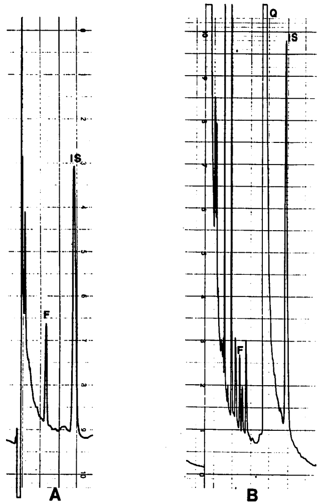
FIG. 1. Chromatograms of serum samples from patients given fentanyl obtained by gas-liquid chromatography on packed (A) or capillary (B) columns. Fentanyl (F) concentrations are 5.8 and 5.7 ng/ml; internal standard (IS) concentrations 25 and 50 ng/ml. Fentanyl retention times were 1.7 and 2.1 min, respectively. The capillary chromatogram was obtained from a patient given quinidine (Q).
