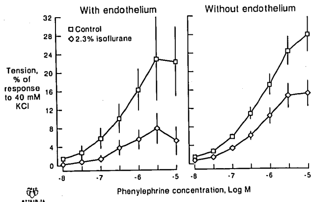
FIG. 4. Cumulative concentration response relationship of rings with and without endothelium exposed to increasing concentrations of phenylephrine ( 10^{-8} to 10^{-5} M). Contractions are expressed as a percentage of the previous contractile response to a standard 40 mM KCl challenge. Phenylephrine evoked concentration-dependent contraction in rings both with and without endothelium. Comparison of integrated areas under the dose-response curves demonstrated that isoflurane significantly depressed tension generation in both rings with endothelium, P < 0.05 , and rings without endothelium, P < 0.005 . Magnitude of the depression of contraction was decreased in the absence of endothelium, P < 0.001 . Data are mean \pm SEM ( n = 6 ).
