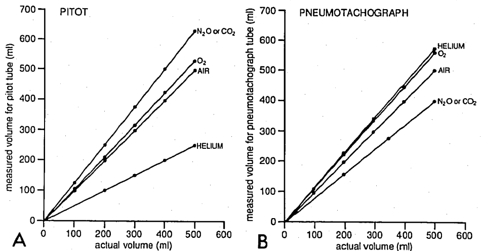
FIG. 4. A comparison of known volumes of helium, oxygen, air, nitrous oxide and carbon dioxide with volumes measured using the modified Pitot tube (A) and pneumotachograph (B).
