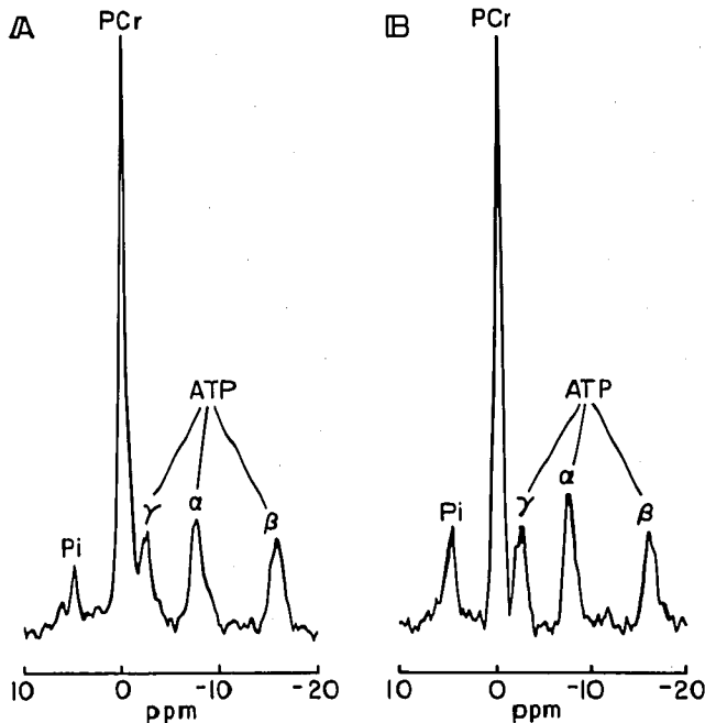
FIG. 1. 31 P NMR spectra of forearm muscles obtained during rest. Spectrum A is from a normal control and spectrum B from an MH-susceptible subject. The different peaks represent relative amounts of phosphorus nuclei from different high-energy phosphate compounds, as labeled. The y-scale has been adjusted so that the PCr peak heights in A and B are equal. Notice that the Pi/PCr is greater in B.
