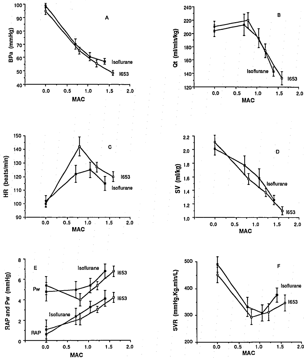
FIG. 1. A. Mean aortic blood pressure (BPa); B. cardiac output ( Q_t ); C. heart rate (HR); D. stroke volume (SV); E. right atrial (RAP) and pulmonary arterial ("wedge") (Pw) pressures; and F. systemic vascular resistance (SVR); in eight swine, conscious and anesthetized with I653 ( \square ) or isoflurane ( \blacksquare ). See table 2 for statistical significance.
