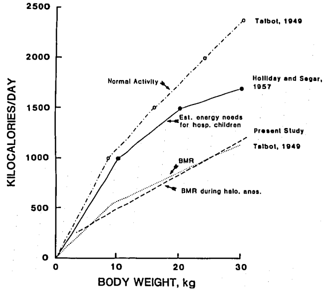
FIG. 4. Daily caloric expenditure in kilocalories related to weight both at basal metabolic rate (BMR) and at normal activity (from Talbot 15 ). Energy needs estimated by Holliday and Segar 6 for hospitalized children are given by continuous line, and those from present study are represented by broken line. (Modified from Holliday MA, Segar WE: The maintenance need for water in parental fluid therapy. Pediatrics 19:823-832, 1957. By permission of Pediatrics.)
