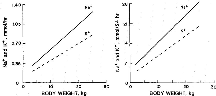
FIG. 3. Average requirement of sodium ( \text{Na}^+ ) and potassium ( \text{K}^+ ) hourly (left diagram) and daily (right diagram) related to weight.
