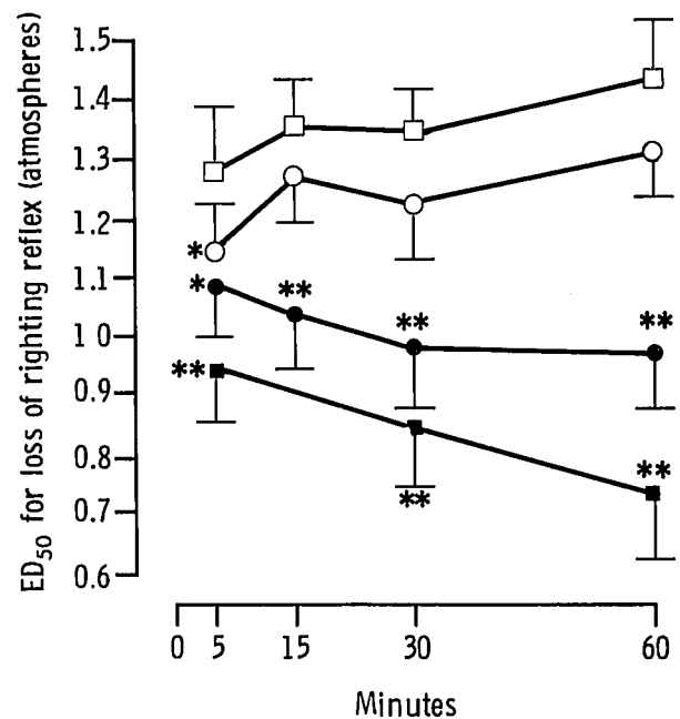
FIG. 3. Time course of the effects of nitrendipine on nitrous oxide anesthesia in mice, when nitrendipine was given 2 h prior to nitrous oxide. ED 50 values for loss of righting reflex were obtained from dose-response lines (fig. 1). Control mice were given a vehicle injection. * P < 0.05 compared with concurrent controls, Chi-squared analysis following probit analysis. □ = Controls, ○ = nitrendipine 10 mg·kg -1 , ● = nitrendipine 50 mg·kg -1 , ■ = nitrendipine 100 mg·kg -1 .
