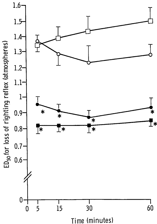
FIG. 2. Time course of the effects of nitrendipine on nitrous oxide anesthesia in mice, when nitrendipine was given 15 min prior to nitrous oxide. ED 50 values for loss of righting reflex were obtained from dose-response lines (fig. 1). Control mice were given a vehicle injection. * P < 0.05 , ** P < 0.01 compared with concurrent controls, Chi-squared analysis following probit analysis. □ = Controls, ○ = nitrendipine 10 mg·kg -1 , ● = nitrendipine 50 mg·kg -1 , ■ = nitrendipine 100 mg·kg -1 .
