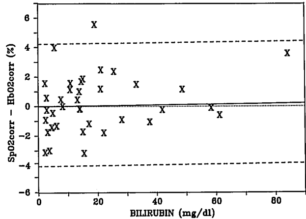
FIG. 3. SpO_2 corr - HbO_2 corr in percent saturation, as a function of total bilirubin level; individual values. Line of regression: SpO_2 corr - HbO_2 corr = 0.0206B - 0.302; r = 0.18 ; NS and 95% prediction limits (---).
