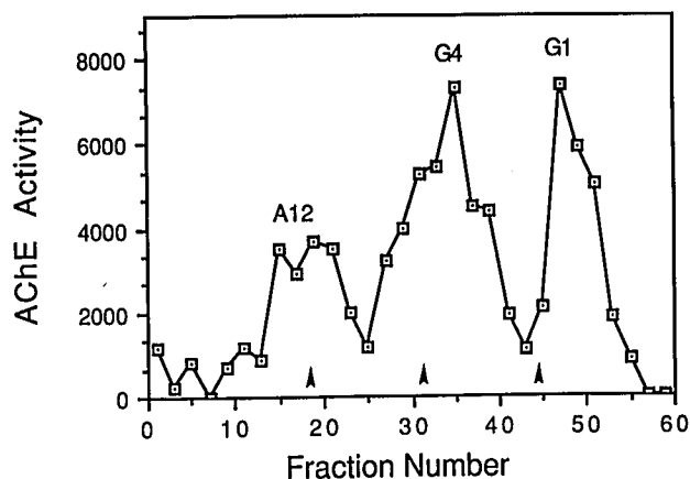
FIG. 2. Separation of the molecular forms of AChE by sucrose gradient centrifugation. Arrows indicate positions of marker enzymes used to determine the size of the molecular forms. Fraction 18, β-galactosidase (16S); fraction 31, catalase (11S); and fraction 44, alkaline phosphatase (6S).
