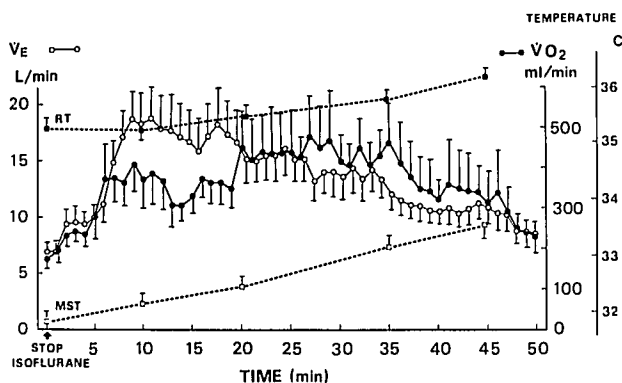
FIG. 1. Mean values ± SEM of rectal temperature (RT), mean skin temperature (MST), minute ventilation ( \dot{V}_E ), and oxygen uptake ( \dot{V}_{O_2} ), after isoflurane discontinuation.
