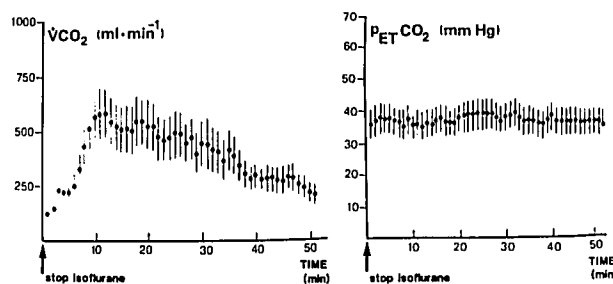
FIG. 2. Mean values ± SEM of CO 2 output ( \dot{V}_{CO_2} ) and end-tidal P CO 2 (PETCO 2 ) after isoflurane discontinuation.
