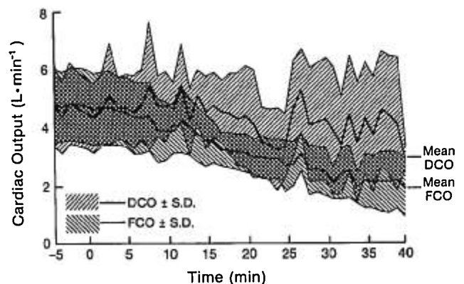
FIG. 1. Cardiac output from 5 min prior to and through hemorrhage (mean \pm SD).
