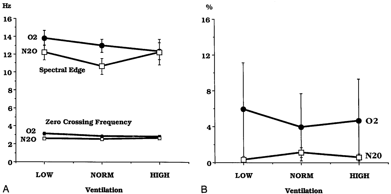
FIG. 4. At 1.24 MAC desflurane there was no difference in either (A) frequency content (as quantitated by SEF and ZXF or (B) degree of suppression (as quantitated by BSR) due to changes in P_{aCO_2} ranging from 26 (LOW) to 58 (HIGH) mmHg.
