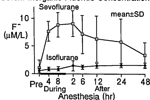
Serum Inorganic Fluoride Concentration
