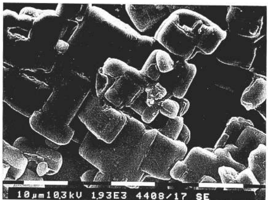
FIG. 1. Scanning electron microscopic (SEM) picture of BAB particles in suspension, after application of a gold layer of 7 nm (electron beam energy 10.3 kV, magnification 1930, Philips SEM). A black or white dash on the dashed black-and-white line indicates a distance of 10 \mu\text{m} .
