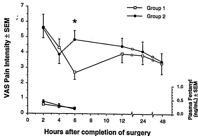
FIG. 2. Mean postoperative visual analogue scale (VAS) pain intensity scores for groups 1 and 2. Zero hours after the completion of surgery corresponds to the time when patients were admitted to the recovery room after the thoracotomy. * P < 0.05 .
