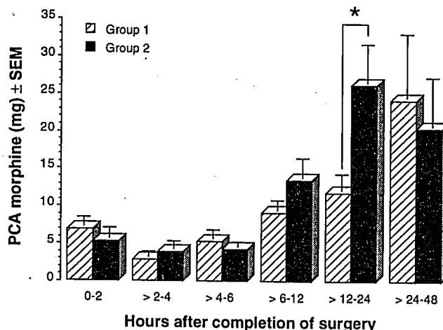
FIG. 3. Mean postoperative PCA morphine consumption for groups 1 and 2. Morphine consumption in the early hours (0–4 h) after the completion of surgery includes both nurse- and patient-administered doses. * P < 0.008 .
