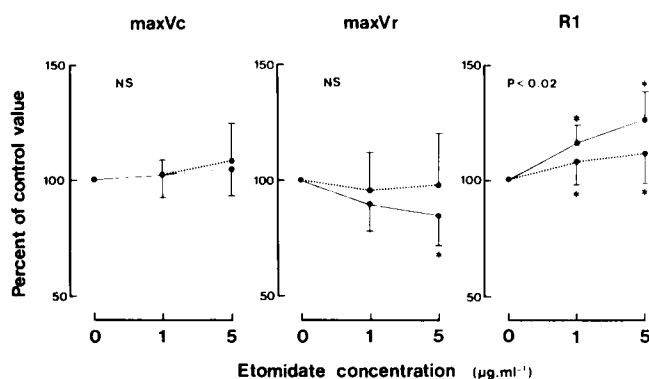
Fig. 2. Comparison of the effects of etomidate on maximum shortening velocity ( _{\max}V_c ), lengthening velocity ( _{\max}V_r ), and contraction-relaxation coupling under low load ( R1 = \text{max}V_c / \text{max}V_r ) of papillary muscles of normal hamsters (solid line) and those with cardiomyopathy (dotted line). Data are mean \pm SD. The P value concerns the between-group differences. * P < .05 versus control values.
