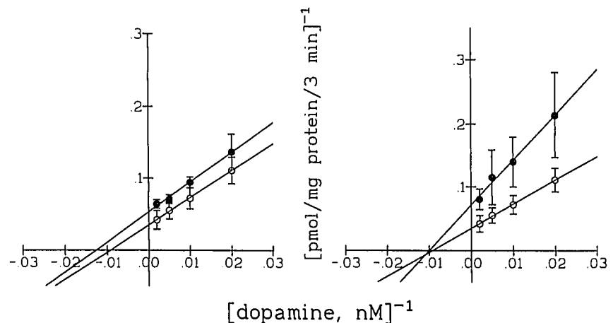
Fig. 4. Double reciprocal plots (Lineweaver-Burke) of experiments in which the concentration of substrate ( ^3\text{H} -DA) is increased from 50 to 500 nM in the presence (solid) or absence (open) of a fixed concentration of anesthetic (see Methods). (Left) Isoflurane data. (Right) Halothane data. Kinetic parameters for these plots are given in table 1.
