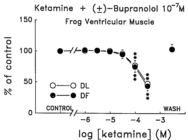
Fig. 9. Effects of ketamine on peak developed force (DF) and peak isotonic shortening (DL) of frog ventricular strips. Values in ketamine (mean \pm SD, n = 8 ) are expressed as percent of control. ** P < 0.01 versus control.
