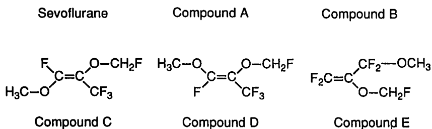
Fig. 1. Chemical structures of sevoflurane and the volatile sevoflurane degradation products.
