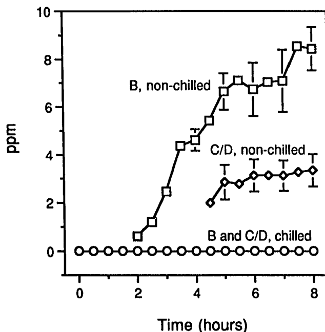
Fig. 5. Concentrations of compound B (open squares) and estimated concentrations of compound C/D (open diamonds) in nonchilled circuits and in circuits in which the soda lime canister was chilled (open circles). No compound B or C/D was detected in circuits employing chilled soda lime. Each point represents the average of the values ( \pm SEM) obtained in three experiments.
