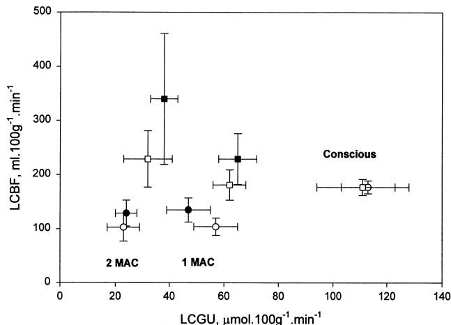
Fig. 1. Relation of local cerebral blood flow (LCBF) to local cerebral glucose utilization (LCGU) (mean values \pm SD, n = 6 ) in auditory cortex (circles) and inferior colliculus (squares). Empty and filled symbols indicate sevoflurane and isoflurane treatment respectively. MAC = minimum alveolar concentration.
