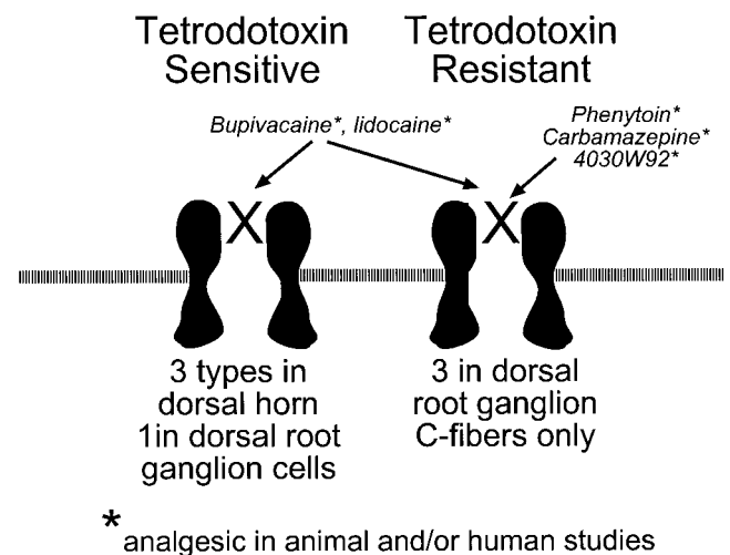
Fig. 2. Summary of the two major classes of sodium channels involved in somatosensory transmission at spinal levels. Drugs that modify each channel are listed, with arrows indicating sites of action. The "X" indicates blockade of the channel. 4030W92 = 2,4-diamino-5-(2,3-dichlorophenyl)-6-fluoromethylpyrimidine. 34
