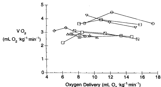
Fig. 2. Relation of oxygen consumption ( VO_2 ) to oxygen delivery ( DO_2 ) in all subjects. A critical DO_2 was not detected.
