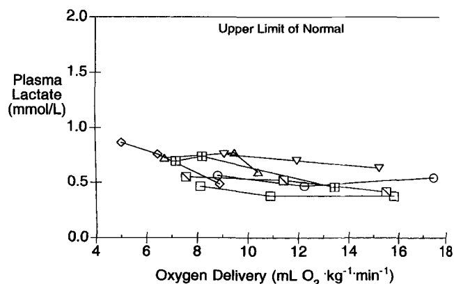
Fig. 4. Plasma lactate concentrations for seven subjects at normal and reduced oxygen delivery ( DO_2 ). No value exceeded the upper limit of normal.
