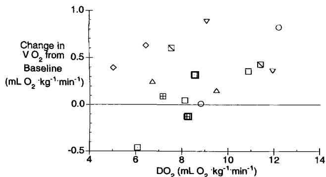
Fig. 3. Change in oxygen consumption ( VO_2 ) from baseline during states of reduced oxygen delivery ( DO_2 ) for each volunteer, represented by a unique symbol. At the lowest DO_2 for each subject, only one subject had a lower VO_2 than at baseline.
