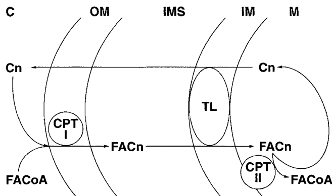
Fig. 1. Schematic of fatty acid transport into mitochondria. FACoA = fatty acyl-CoA; FACn = fatty acylcarnitine; CPT = carnitine palmitoyl transferase; Cn = carnitine; C = cytoplasm; OM = outer mitochondrial membrane; IMS = intermembrane space; IM = inner mitochondrial membrane; M = matrix; TL = carnitine-acylcarnitine translocase.
