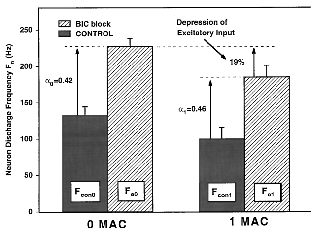
Fig. 2. Method used to quantify the effects of halothane on overall synaptic neurotransmission (data from neuron shown in fig. 1). Values for peak neuronal discharge frequency ( F_n ) before bicuculline (BIC) block ( F_{con} ) and during BIC block ( F_e ) at each minimum alveolar concentration (MAC) level were used to calculate the inhibitory factor \alpha . During BIC block ( \alpha = 0 ), 1 MAC halothane reduced the overall excitatory drive by 19%. Coefficient of variations are (left to right): 1.1, 2.0, 1.5, and 2.7%.
