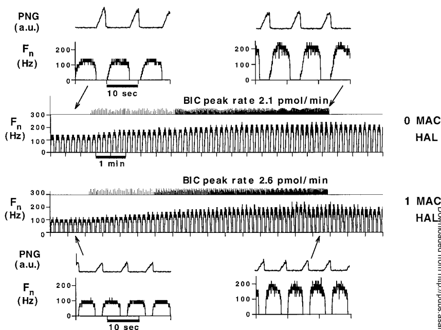
Fig. 1. Response of an expiratory neuron to picrojection of the GABA A antagonist bicuculline (BIC) at 0 and 1 minimum alveolar concentration (MAC) halothane (HAL). The picrojection response curves to BIC (see picrojection marker) are shown in the middle traces as rate-meter recordings of the neuronal discharge frequency ( F_n ). The top and bottom records show time-expanded views of the phrenic neurogram (PNG; arbitrary units [a.u.]) and simultaneous neuronal rate-meter recordings during both the preejection control period (left traces) and maximal increase of the neuronal discharge frequency (right traces).
