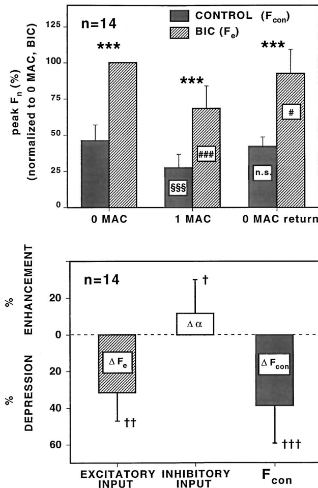
Fig. 3. Pooled summary data of study 1. (Top) Mean values \pm SD of normalized peak neuronal discharge frequency ( F_n ; %) before ( F_{con} ) and during ( F_e ) maximal GABAergic block with bicuculline (BIC) for the 0 minimum alveolar concentration (MAC), 1 MAC, and 0 MAC end-control doses for 14 neurons. At all MAC levels, F_e was significantly greater than F_{con} ( ***P < 0.001 ). Halothane, 1 MAC, caused a significant reduction of F_{con} (SSSP < 0.001 ) and F_e (###P < 0.001 ). The 0-MAC end-control values for F_{con} were not different (not significant) from the initial 0 MAC values, indicating stability of the preparation. A small but significant decline in F_e ( 7.4 \pm 16.7\% ) of the end control was present ( \#P < 0.05 ). (Bottom) Mean depression \pm SD of overall excitatory drive, ( \Delta F_e ), mean enhancement of inhibitory neurotransmission ( \Delta \alpha ), and the resulting mean depression of control frequency ( \Delta F_{con} ) by 1 MAC halothane in 14 neurons. ( \dagger P < 0.05 , \dagger\dagger P < 0.01 , \dagger\dagger\dagger P < 0.001 relative to no change.)
