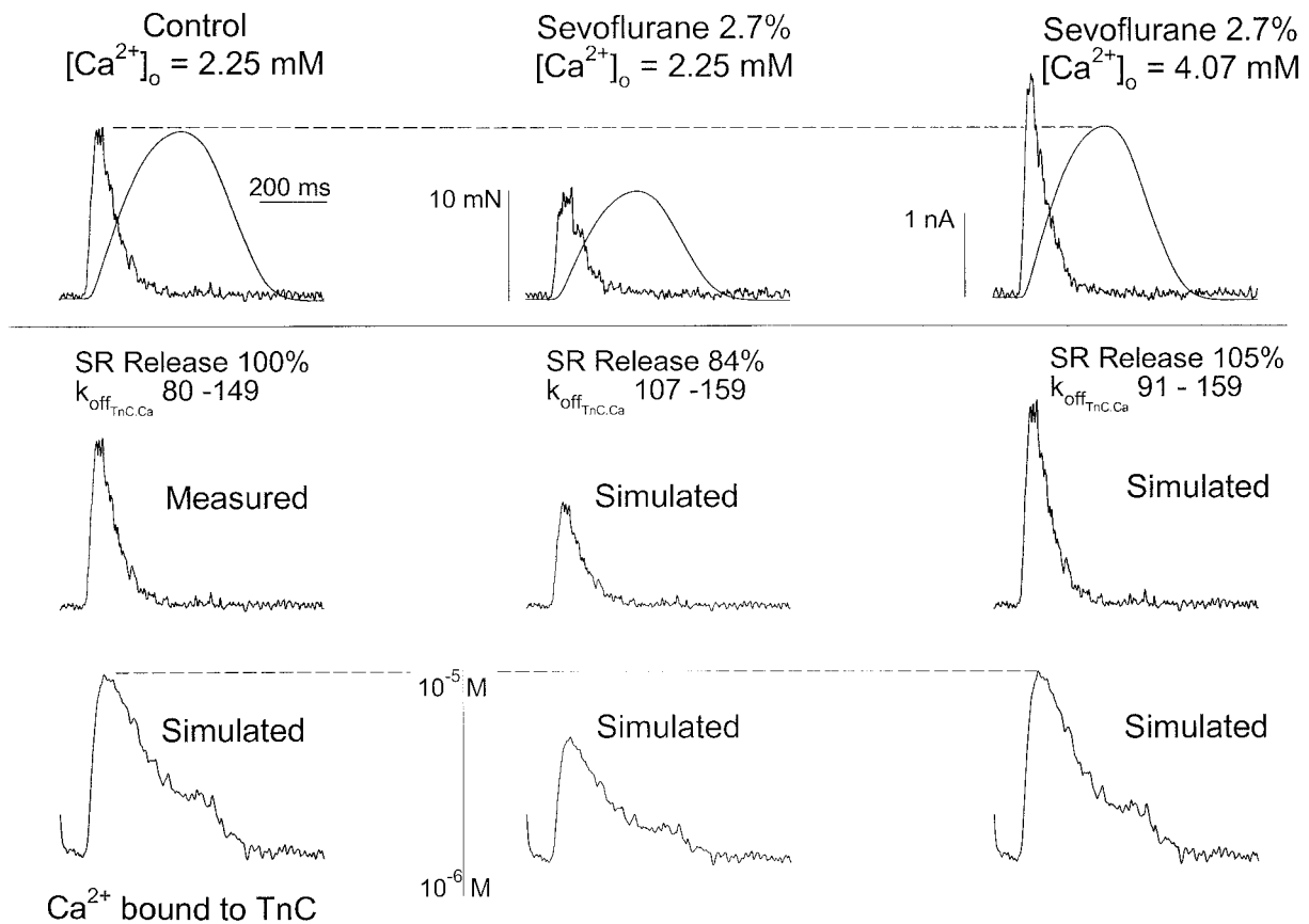
Fig. 5. Analysis of isometric \text{Ca}^{2+} back-titration experiment. ( Top ) Aequorin luminescence and force traces as a function of time in a typical \text{Ca}^{2+} back-titration experiment. Sixty-four twitch contractions were averaged. ( Middle ) Traces of aequorin luminescence obtained by computational simulation, except where marked "measured." ( Bottom ) Calculated traces of \text{Ca}^{2+} occupancy of troponin C. See text for details. SR = sarcoplasmic reticulum.
