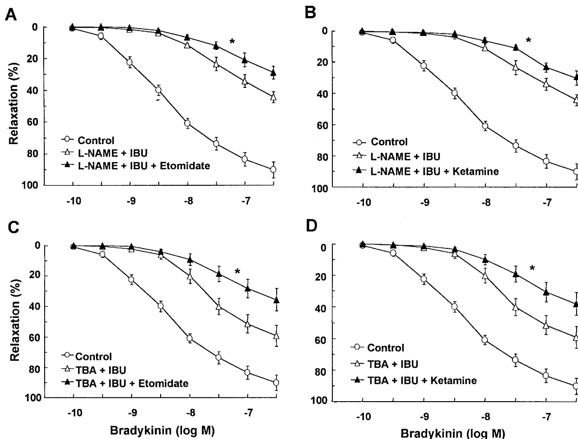
Fig. 5. Concentration–effect curves summarizing the effects of etomidate ( 10^{-4} M) and ketamine ( 10^{-4} M) on the L-NAME-resistant (A and B) and TBA-resistant (C and D) components of bradykinin-induced relaxation in ibuprofen (IBU)-pretreated rings. Pulmonary arterial rings were precontracted to the ED_{50} level of tension with phenylephrine. Etomidate and ketamine attenuated (* P < 0.05 ) the L-NAME-resistant and TBA-resistant relaxation.
