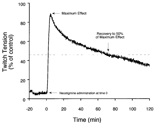
Fig. 1. Neuromuscular response data from one subject. Neostigmine, 70 \mu\text{g}/\text{kg} , was administered at time zero. Control twitch tension was obtained after the volunteer had attained and stabilized at the desired study temperature and before vecuronium administration.
