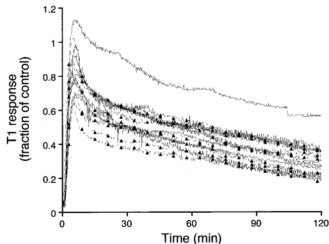
Fig. 2. Neuromuscular response data following neostigmine administration for all subjects. Neostigmine, 70 \mu\text{g}/\text{kg} , was administered at time zero. T1 control was the amplitude of the first response (T1) in the stable train-of-four sequence recorded just before the first administration of vecuronium. Data for normothermia are identified by the dashed lines and solid triangles.
