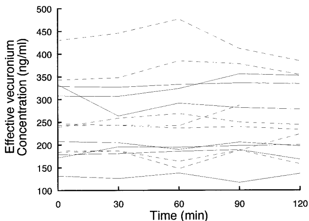
Fig. 5. Effective plasma concentrations of vecuronium versus time for the 2 h following neostigmine administration in normothermic (dashed lines) and hypothermic volunteers (solid lines). The effective concentration is the sum of vecuronium plus that of its active metabolite, 3-desacetylvecuronium. Concentrations of 3-desacetylvecuronium were multiplied by 0.83 to reflect its potency relative to vecuronium. 7
