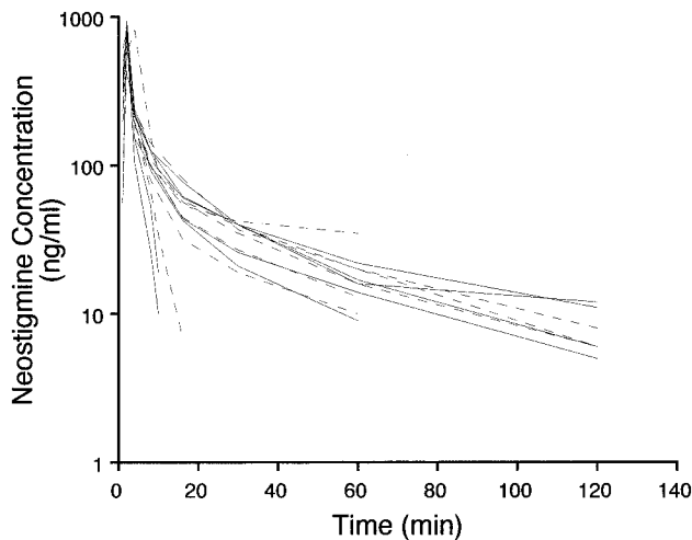
Fig. 3. Plasma concentration versus time data for neostigmine in normothermic (dashed lines) and hypothermic volunteers (solid lines).
