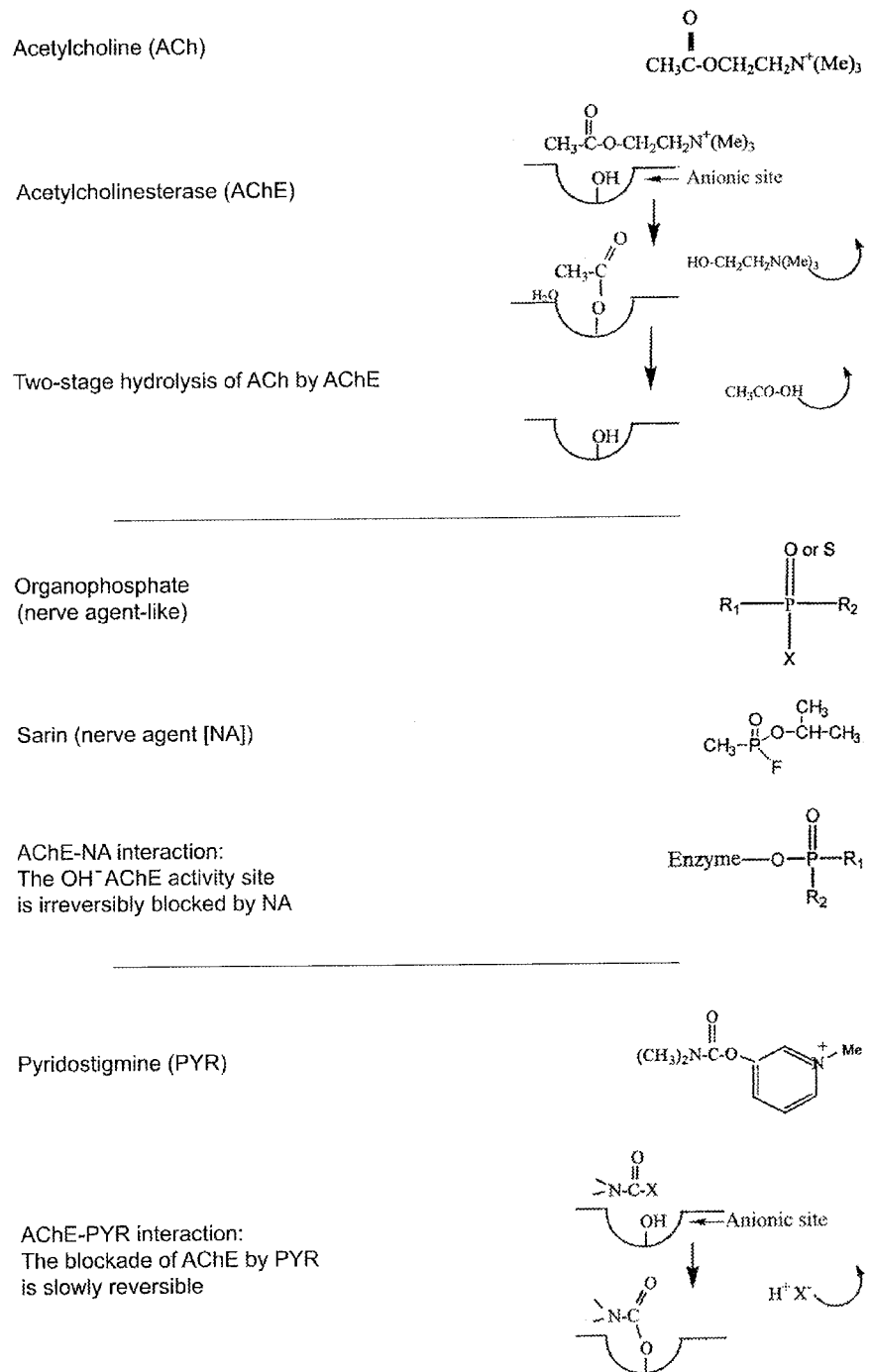
Fig. 1. Chemical interactions between acetylcholinesterase and acetylcholine, organophosphate, nerve agents, and pyridostigmine.
