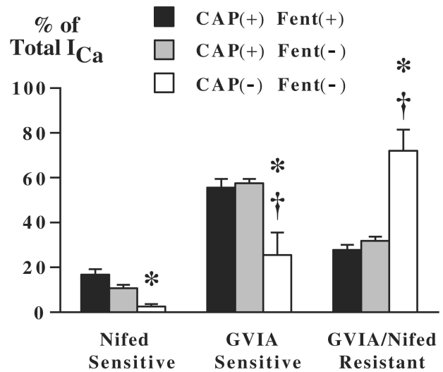
Fig. 6. The percentages of whole cell \text{Ca}^{2+} current ( I_{Ca} ) sensitive to the L-type \text{Ca}^{2+} channel blocker nifedipine (Nifed, 10 \mu\text{M} ), the N-type \text{Ca}^{2+} channel blocker \omega -conotoxin GVIA (GVIA, 1 \mu\text{M} ), and the percentage that was resistant to a combination of both. CAP (+) = capsaicin responsive; CAP (-) = capsaicin unresponsive; Fent (+) = fentanyl sensitive; Fent (-) = fentanyl insensitive. The CAP-unresponsive, fentanyl-insensitive cells ( n = 3 ) had significantly less L- and N-type I_{Ca} and a greater percentage of I_{Ca} that was resistant to both blockers ( *P < 0.01 vs. CAP-sensitive, fentanyl-sensitive cells, n = 4 ; \dagger P < 0.001 vs. CAP-sensitive, fentanyl-insensitive cells, n = 6 ).
