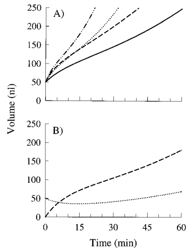
Fig. 3. (A) Time course of embolism growth for 50-nl cerebral oxygen bubbles during 70% Xe-30% O 2 delivery at 37°C. L_o/R_o = 0 (dashed line), 2.6 (solid line), 10 (dotted line), 20 (dashed-dotted line). (B) Individual gas volumes for xenon (dashed line) and oxygen (dotted line) for L_o/R_o = 2.6 .
