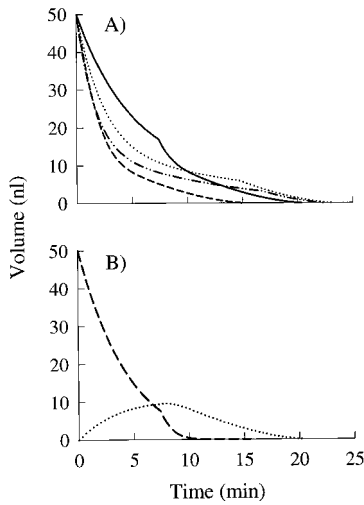
Fig. 1. (A) Time course of embolism reabsorption for 50-nl cerebral xenon bubbles during oxygen delivery at 37°C. L_o/R_o = 0 (dashed line), 2.6 (solid line), 10 (dotted line), 20 (dashed-dotted line). The kink in the curves occurs at the transition from cylindrical to spherical solutions. (B) Individual gas volumes for xenon (dashed line) and oxygen (dotted line) for L_o/R_o = 2.6 .
