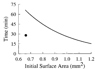
Fig. 4. Predicted time required for a 50-nl xenon cerebral embolism bubble to double its volume at 37°C during 70% Xe-30% O 2 delivery. The single point (dot) denotes a spherical bubble growing as a sphere. Elongating bubbles ( L_o/R_o > 0 ) growing at fixed radius appear in the curve.
