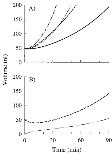
Fig. 2. (A) Time course of embolism growth for 50-nl cerebral xenon bubbles during 70% Xe-30% O 2 delivery at 37°C. L_o/R_o = 0 (dashed line), 2.6 (solid line), 10 (dotted line), 20 (dashed-dotted line). (B) Individual gas volumes for xenon (dashed line) and oxygen (dotted line) for L_o/R_o = 2.6 .
