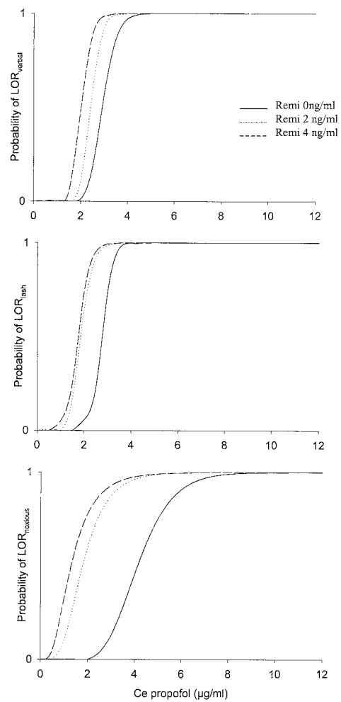
Fig. 5. Probability of loss of response to verbal commend ( LOR_{verbal} ), eyelash reflex ( LOR_{lash} ), and a tetanic electrical stimulus ( LOR_{noxious} ) as a function of the propofol effect-site concentration (Ce). Data from the 0 ng/ml remifentanil (Remi) group are presented as a solid line, data from the 2 ng/ml remifentanil group as a dotted line, and data from the 4 ng/ml remifentanil group as a dashed line.
