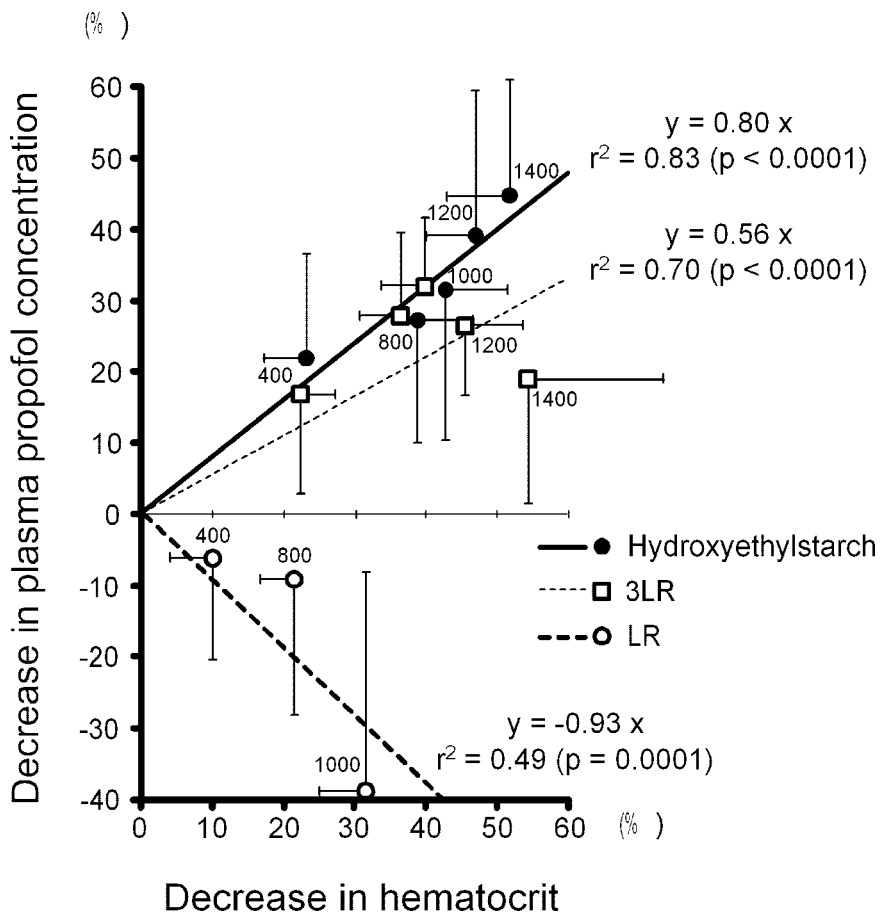
Fig. 4. Relation between the decrease in hematocrit [100 × (Hematocrit at Baseline - Hematocrit)/Hematocrit at Baseline] and the decrease in plasma propofol concentration [100 × (Plasma Propofol Concentration at Baseline - Plasma Propofol Concentration at Baseline)/Plasma Propofol Concentration at Baseline] in each fluid infusion. Each point represents the mean and SD at each hemorrhage and infusion step (the numbers shown in the figure give the total blood-fluid exchange volume in each group). The linear regression analyses were based on raw data in each group (raw data are not shown). The linear regression equations are y = -0.93x, r 2 = 0.49 (P = 0.0001) in the lactated Ringer's solution (LR) group, y = 0.80x, r 2 = 0.83 (P < 0.0001) in the hydroxyethyl starch group, and y = 0.56x, r 2 = 0.70 (P < 0.0001) in the threefold lactated Ringer's solution (3LR) group.
