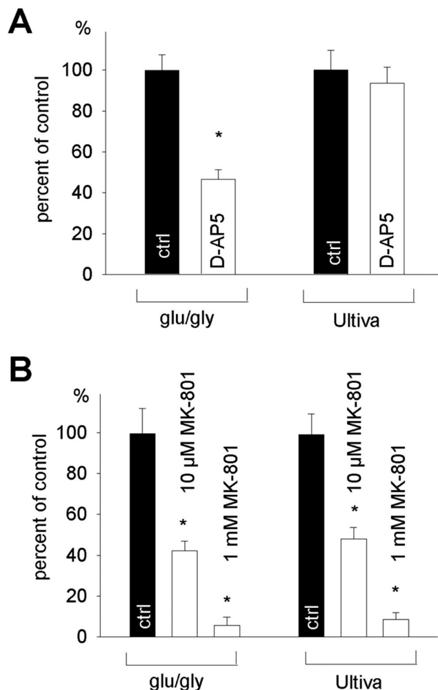
Fig. 5. (A) The competitive glutamate binding site antagonist D-AP5 (1 mM; white bars) inhibits glutamate/glycine-induced currents ( EC_{50} ) ( * P < 0.05 ) but does not affect Ultiva®-induced (remifentanil 0.1 mM plus glycine 3.1 mM) responses ( n > 10 ; vertical bars \pm SEMs). (B) The noncompetitive N -methyl-D-aspartate receptor channel pore blocker MK-801 inhibits N -methyl-D-aspartate receptor responses (NR1A/2A) to Ultiva® (remifentanil 0.1 mM plus glycine 3.1 mM) and glutamate/glycine ( EC_{50} ) in a concentration-dependent manner ( * P < 0.05 ; n = 10 ; vertical bars \pm SEMs).
