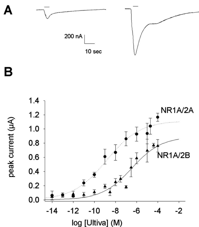
Fig. 2. (A) Representative traces of N -methyl-D-aspartate receptor responses induced by different concentrations of Ultiva ® (left trace, 0.25 nM; right trace, 0.24 μM) in oocytes expressing NR1A/NR2A receptors; black line shows duration of Ultiva ® application. (B) Ultiva ® evokes inward currents in a concentration-dependent manner in oocytes expressing NR1A/2A (EC 50 = 3.5 nM) (circles) or NR1A/2B (EC 50 = 0.8 μM) receptors (n = 10 for each data point; means ± SEMs).
