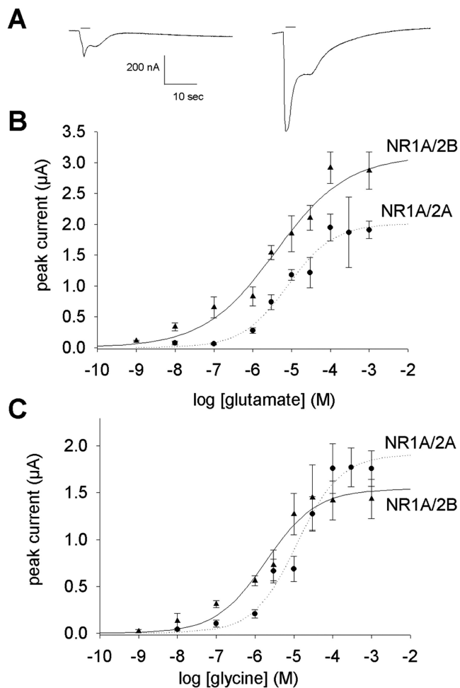
Fig. 1. NR1A/NR2A and NR1A/NR2B N-methyl-D-aspartate receptors expressed recombinantly in Xenopus laevis oocytes. (A) Representative traces of N-methyl-D-aspartate receptor responses induced by different concentrations of glutamate (left trace, 0.1 μM; right trace, 0.1 mM) in the presence of 10 μM glycine in oocytes expressing NR1A/NR2B receptors; black line shows duration of agonist application. (B) Glutamate, in the presence of 0.1 μM glycine, evokes inward currents in a concentration-dependent manner in oocytes expressing NR1A/2A (EC 50 = 8.0 μM) (circles) or NR1A/2B (EC 50 = 3.9 μM) (triangles) receptors (n = 10 for each data point; means ± SEMs). (C) Glycine, in the presence of EC 50 glutamate, evokes inward currents in a concentration-dependent manner in oocytes expressing NR1A/2A (EC 50 = 12 μM) (circles) or NR1A/2B (EC 50 = 1.9 μM) (triangles) receptors (n = 10 for each data point; means ± SEMs).
