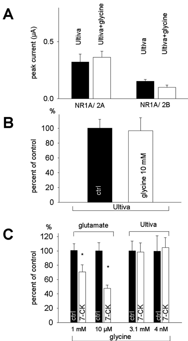
Fig. 4. (A) Addition of glycine (10 μM) to Ultiva® (white bars; 24 nM remifentanil plus 0.4 μM glycine) does not induce an additive effect on either receptor subtype combination compared with Ultiva® (black bars; 24 nM remifentanil plus 0.4 μM glycine alone) ( P > 0.05 ; n = 10 ; vertical bars \pm SEMs). (B) Preapplication of a saturating glycine concentration (10 mM; white bar) before application of Ultiva® (remifentanil 0.24 nM plus glycine 4 nM) does not enhance Ultiva®-induced currents in N -methyl-D-aspartate receptors (NR1A/2A) ( n = 10 ; vertical bars \pm SEMs). (C) Glutamate/glycine-evoked N -methyl-D-aspartate receptor responses (NR1A/2A) are inhibited by the glycine site antagonist 7-CK (5 μM; white bars) in a glycine concentration-dependent manner. Responses to both Ultiva® concentrations (remifentanil 0.1 mM plus glycine 3.1 mM and remifentanil 0.25 nM plus glycine 4 nM) are not affected by 7-CK ( * P < 0.05 ; n = 10 ; vertical bars \pm SEMs).
