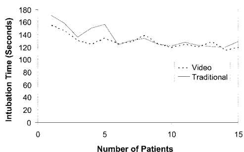
Fig. 2. Mean cumulative time required by residents in each group to complete an intubation or to fail to intubate for each patient number.
