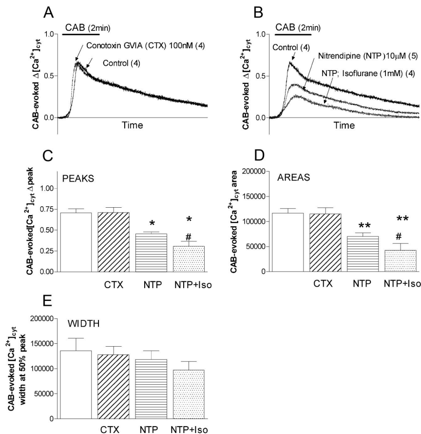
Fig. 3. Nitrendipine a L-type Ca^{2+} channel blocker reduces the carbachol-evoked [Ca^{2+}]_{cyt} transient but does not eliminate the isoflurane sensitivity of the carbachol-evoked [Ca^{2+}]_{cyt} transient. The application of the calcium channel blocker was started 10 min before the carbachol (CAB) stimulation; and the application of isoflurane (1 mM) 5 min before the carbachol stimulation was 2 min. (A) The averaged carbachol-evoked [Ca^{2+}]_{cyt} transients in the absence and presence of \omega -conotoxin GVIA (CTX, 100 nM). (B) The averaged carbachol-evoked [Ca^{2+}]_{cyt} transients in the absence and presence of nitrendipine (NTP, 10 \mu M); and of NTP plus 1 mM isoflurane (Iso). The corresponding measurements: peaks (C), areas (D), and widths at 50% peak height (E) of the carbachol-evoked [Ca^{2+}]_{cyt} transient in the absence and presence of either \omega -conotoxin GVIA, NTP, and NTP plus isoflurane (NTP+Iso). Units: Peaks ( \Delta ratio 340/380); Areas (ratio 340/380 * ms) and Width at 50% peak (ms). The horizontal bars in A and B indicate a 2-min period. The results were expressed as mean \pm SEM in panels A and B and as mean \pm SEM in panels C, D, and E. Statistically significant differences from control are indicated as follows: * P < 0.001 , ** P < 0.01 ; and statistically significant differences from the NTP group are indicated as follows: # P < 0.05 (Newman-Keuls test). The baseline values (absolute ratio values before the addition of carbachol) were not statistically different ( P > 0.05 ) between control and the treated groups (data not shown).
